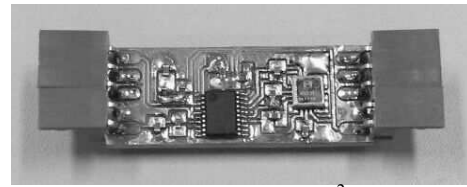
Fig. 10 Sensor chip ( 14 \times 38 \text{ mm}^2 ) measuring the gravity vector and transmitting the measured data to the host PC via an I 2 C bus line.
