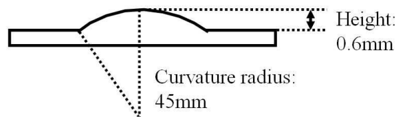
Figure 10. Base with hemispherical bump.
