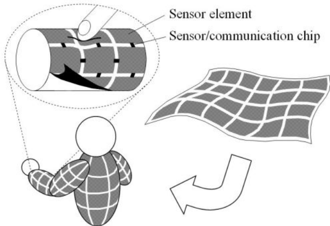
Figure 1. Robot skin composed of proposed sensor elements. It is soft, stretchable, and capable to cover a large area easily.
