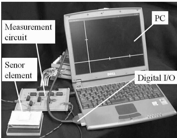
Figure 8. Experimental setup.
