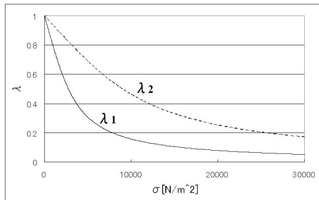
Figure 5. Relationship between surface stress \sigma and extension ratio \lambda_n . Soft layer \lambda_1 is more easily compressed than hard layer \lambda_2 .
