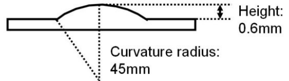
Fig. 8 Cross-section of the curved base.
