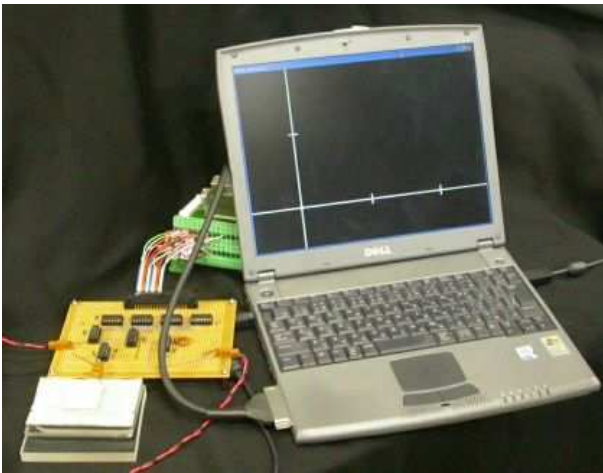
Fig. 6 Experimental setup.
